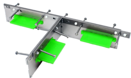
Durashield " T " junction armour joint
