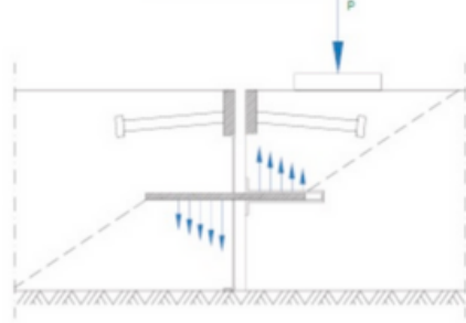
Figure 1. Load Transfer
